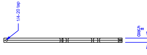
VERTICAL SECTION
