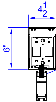
VERTICAL SECTION
