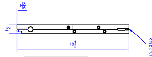
CENTER HUNG ARM
